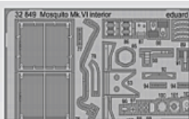
32849 Mosquito Mk.VI interior 1/32 Tamiya
