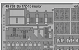
49738 Do 17Z-10 interior 1/48 ICM
