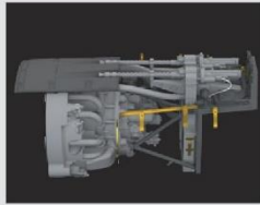
648392 Fw 190A-5 fuselage guns 1/48 Eduard
