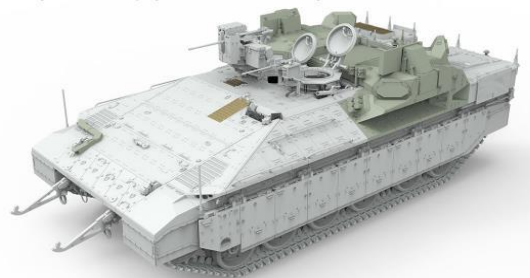
☆ “雌虎”重型装甲运输车搭载“战利品”主动防御系统形态 Namer Heavy APC w/Trophy Active Protection System
