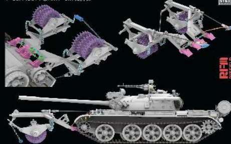
T-55A Mod.1981 with KMT-5M Mine Roller
